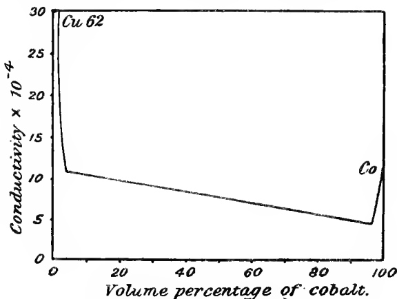
FIG. 86.—Conductivity of copper-cobalt alloys.
